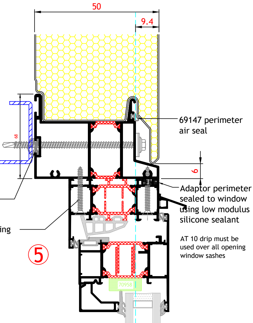
C/L Column Top Hat - Condition Typical Window Outside Elevation
